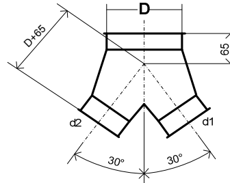
Hosenrohr 30° Culotte 30°
